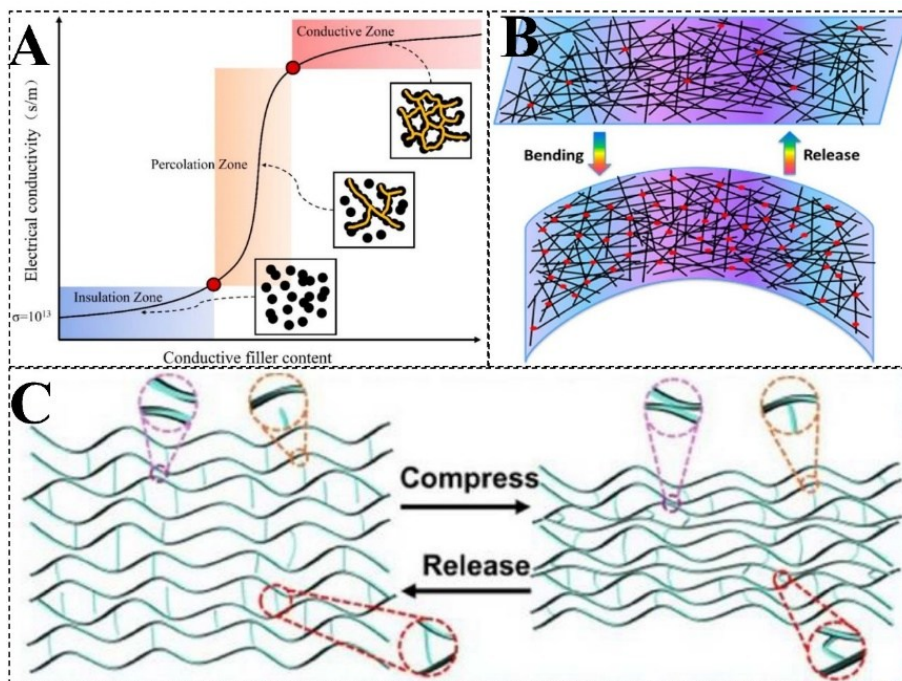
Fig. 5. Schematic illustration of representative strain sensing mechanisms in biomass-derived carbon composites. (A) Percolation model for conductivity of composites (Zhang et al. 2024c). (B) Schematic representation showing the internal network changes of the carbon paper/PDMS composite before and during applied strain. The carbon fibers are illustrated as black lines, and red points highlight breaks or gaps that form in the conductive pathways (Reprinted with permission from Li et al. 2016, American Chemical Society). (C) Compression mechanism of biocarbon aerogel (Reprinted with permission from Jiang et al. 2026, Wiley).
