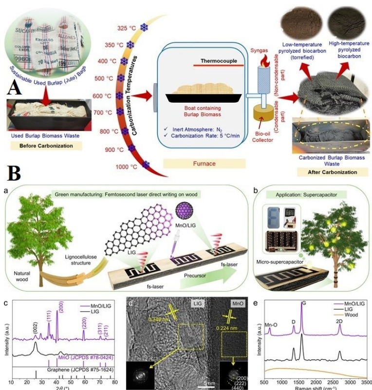
Fig. 3. Typical carbonization pathways of lignocellulosic biomass. (A) Carbonization route for the production of burlap-derived biocarbon (Tripathi et al. 2022). (B) Laser-induced graphitization (LIG) on wood surfaces (Kim et al. 2024)
