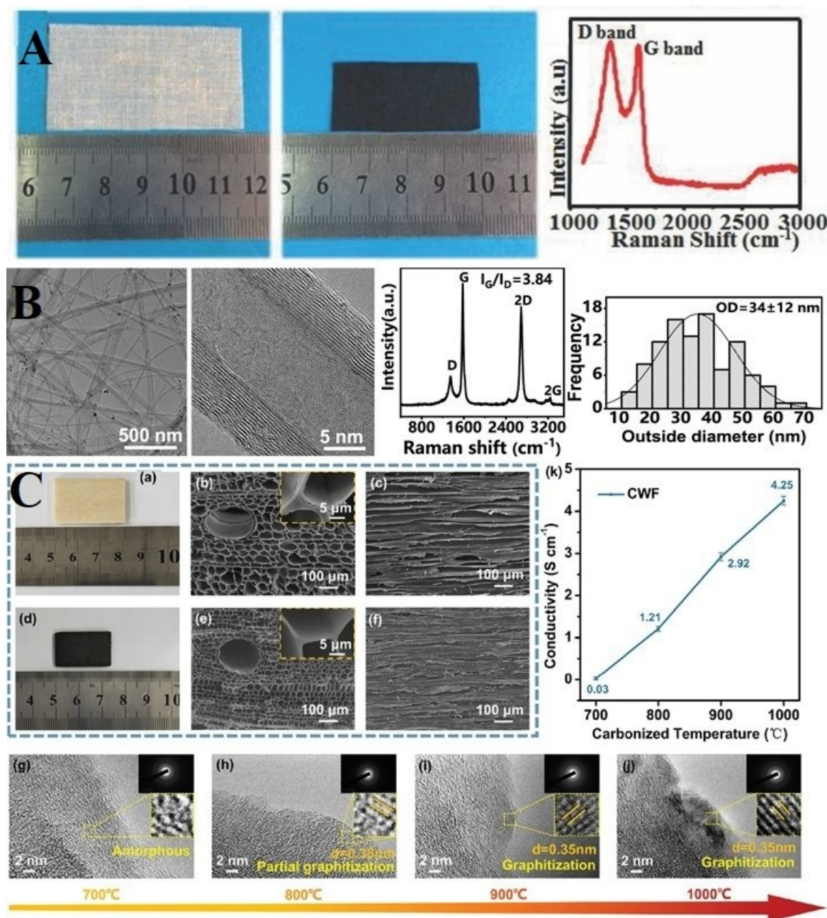
Fig. 4. Morphological diversity of biomass-derived conductive biocarbons. (A) Carbonized cotton fabrics retaining the woven textile structure (Reprinted with permission from Zhang et al. 2017, Wiley). (B) Structures of the lignin-derived carbon nanotube fiber (Liu et al. 2022). (C) Structural and conductive properties of carbonized wood frameworks (CWF) (Reprinted with permission from Ji et al. 2022, Wiley)
