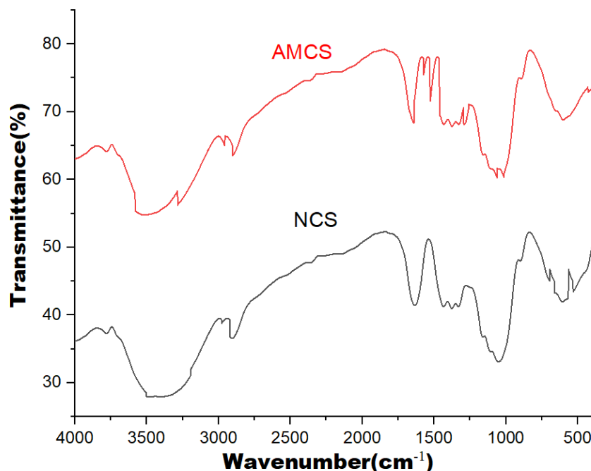
Fig. 5. FTIR Analysis of native cocoyam starch (NCS); and acid-modified cocoyam starch (AMCS)
