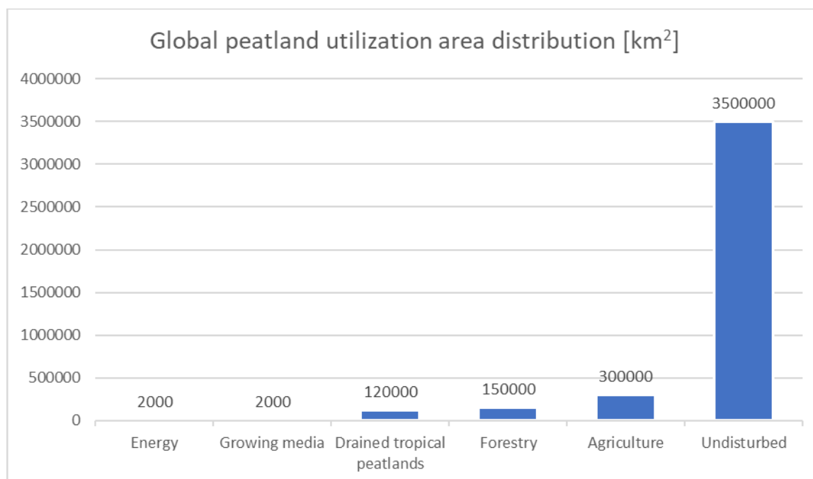
Fig. 2. Global peatland utilization area distribution (World Energy Council 2013; Clarke and Rieley 2010)
