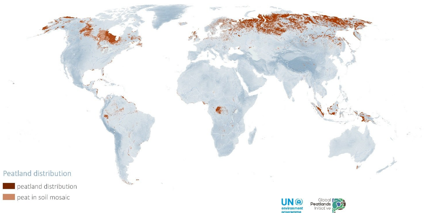
Fig. 1. The Global peatland Map 2.0 (Adapted from United Nations Environment Programme 2021).
