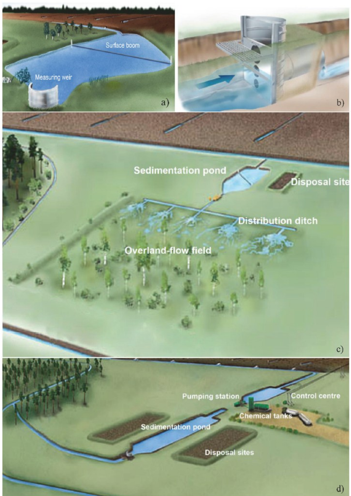
Fig. 7. The most commonly used water treatment methods for peat extraction areas in Finland. a) Constructed sedimentation pond, b) peak runoff control dam, c) overland flow field and d) chemical purification (Heiderscheidt 2016)
