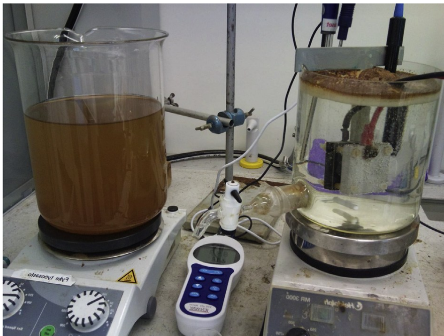
Fig. 8. PBDW from a Finnish peat bog before and after batch-EC treatment (Kuokkanen et al. 2015)
