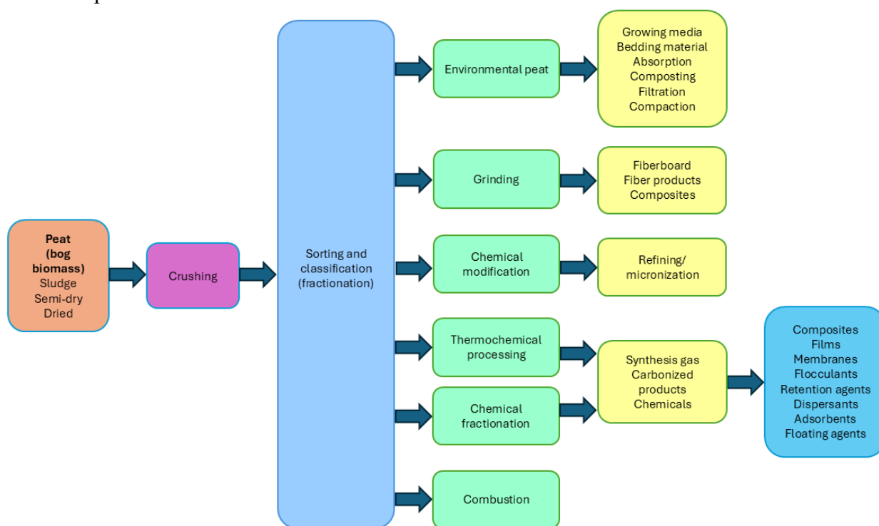
Fig. 3. Refining of peat and bog biomass. Adapted from Arvola (2015).
