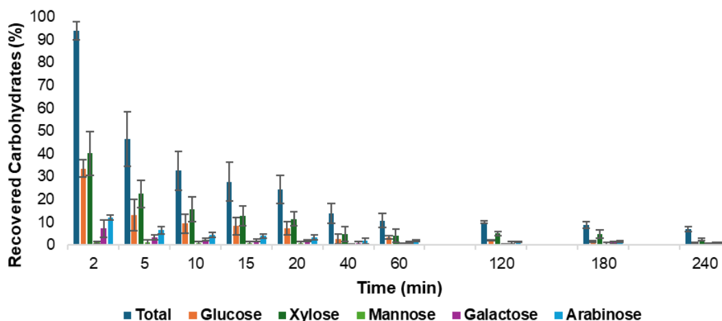
Fig. 2. Carbohydrate concentration (%) in the dry material of the liquor extracts over time in a birch treated with 1:2 ( \text{NaIO}_4 : biomass) mass ratio; Total concentration of detected carbohydrates in the extracted material is shown in dark blue
