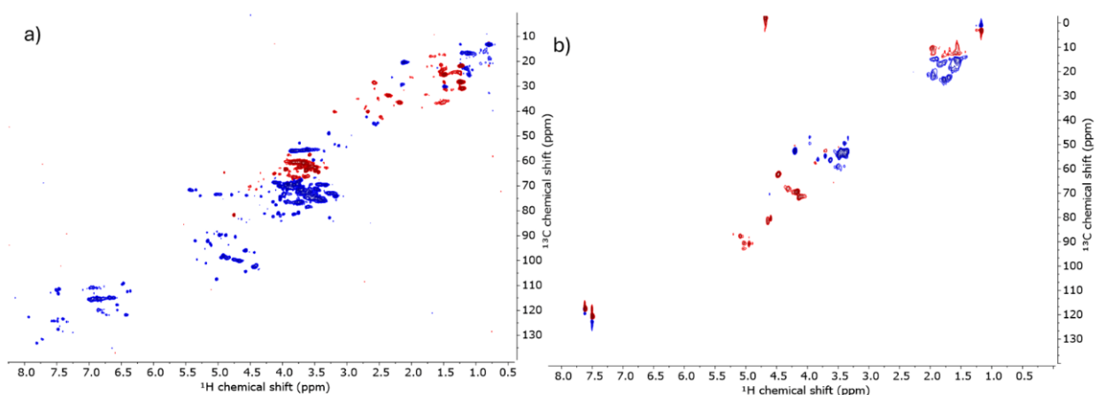
Fig. 4. ^1\text{H} - ^{13}\text{C} HQSC NMR spectra of birch for a) reference water-extracted sample for 60 min and b) periodate extracted sample after treatment for 60 min, 1:2 ratio ( \text{NaIO}_4 : biomass), Red and blue contours represent signals with positive and negative phases, respectively, corresponding to \text{CH}/\text{CH}_3 and \text{CH}_2 groups in the multiplicity-edited HSQC experiment.
