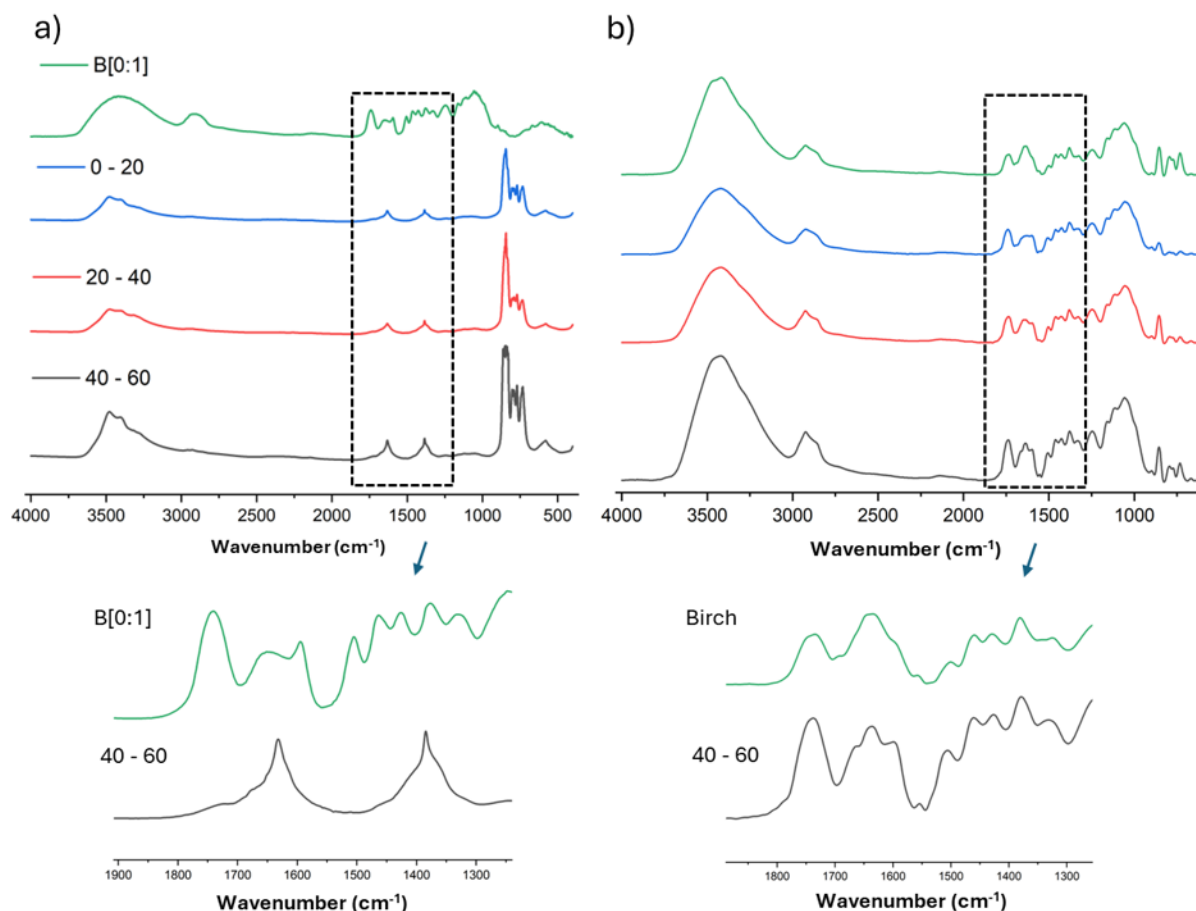
Fig. 5. FTIR spectra of a) liquor samples extracted with only water (B[0:1]) and periodate \text{NaIO}_4 :biomass ratio 1:2 for different treatment times (0 to 60 min), followed by \text{NaBH}_4 reduction; b) the remaining solid fractions
