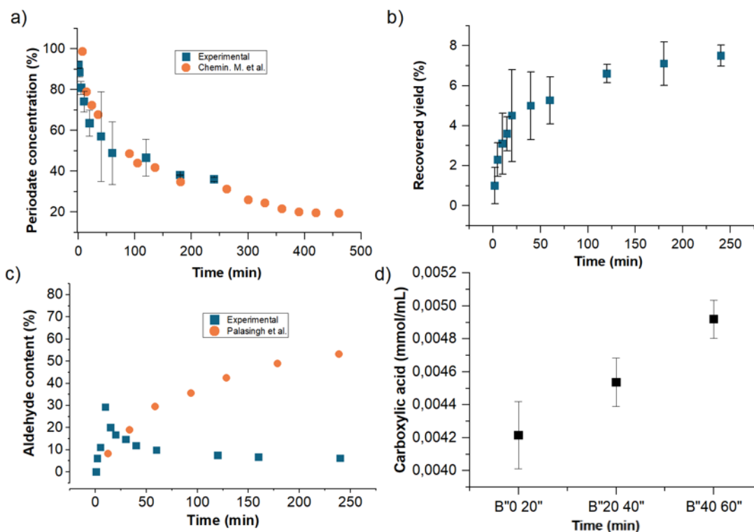
Fig. 1. a) Periodate concentration (as % of total oxidizing liquor) during oxidation of birch, mass ratio 1:2 ( \text{NaIO}_4 : biomass) compared to the results obtained by Chemin M. et al. (2016); b) yield of material extracted over the studied oxidation time; c) Aldehyde concentration detected in the extracted material (as % of the total dry mass over time compared to that obtained by Palasingh C. et al. (2022); and d) carboxylic acid amounts measured in extracted material over time for the same \text{NaIO}_4 : biomass mass ratio
