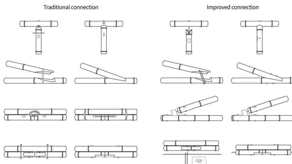
Fig. 5. Modern connection methods
