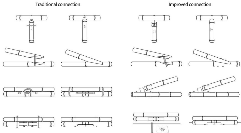
Fig. 5. Modern connection methods
