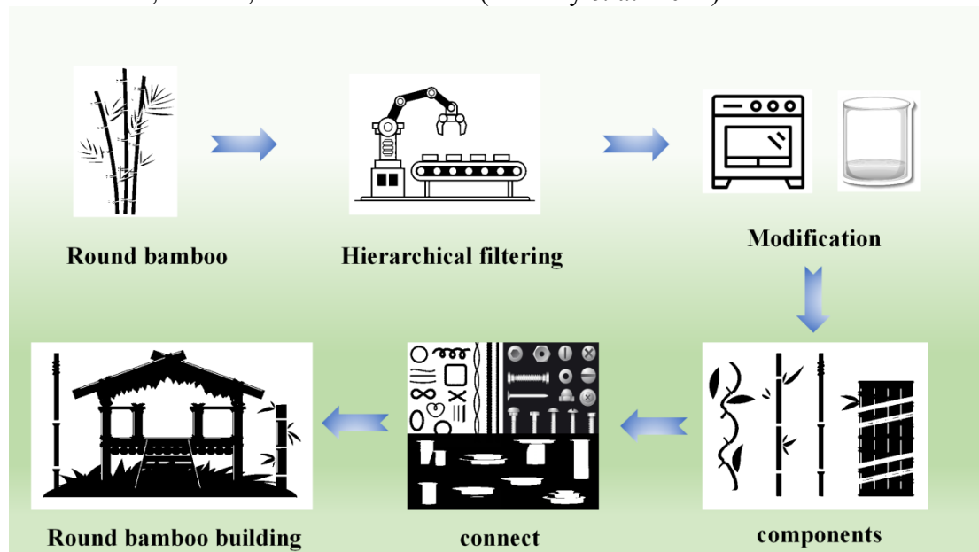
Fig. 2. The construction process of round bamboo buildings
