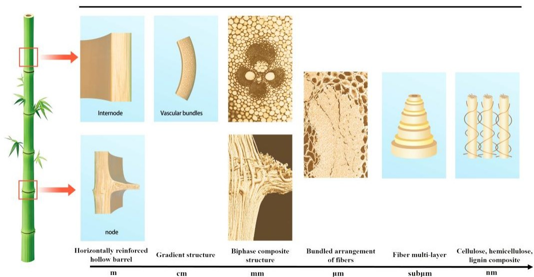
Fig. 1. The multilevel structure of natural bamboo from macro to micro
