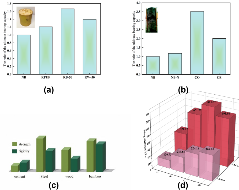
Fig. 3. (a) and (b): The ratio of the ultimate bearing capacity of the filled bamboos with different materials to the natural bamboos, NB: nature bamboo, RPUF: Polyurethane filling, RB-50\RW-50: 50:50 percent of polyurethane and 50% of bamboo \wood strips each; NB-N: nature bamboo with node; CO: Concrete filling; CE: Cement mortar filling; (c) Ratio of strength and stiffness of bamboo to other materials, (d) Ring stiffness of rice husk foam-filled round bamboo, A: nature bamboo; B: Modified round bamboo; C: nature bamboo with node; and D: Modified round bamboo with node (Hildayanti et al. 2023; Zhao et al. 2023; Su et al. 2020).
