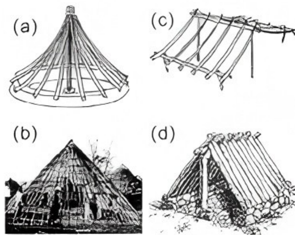
Fig. 6. (a),(b) Primitive bamboo hut I, (c),(d) Primitive bamboo hut II (from www.pinterest.com )
