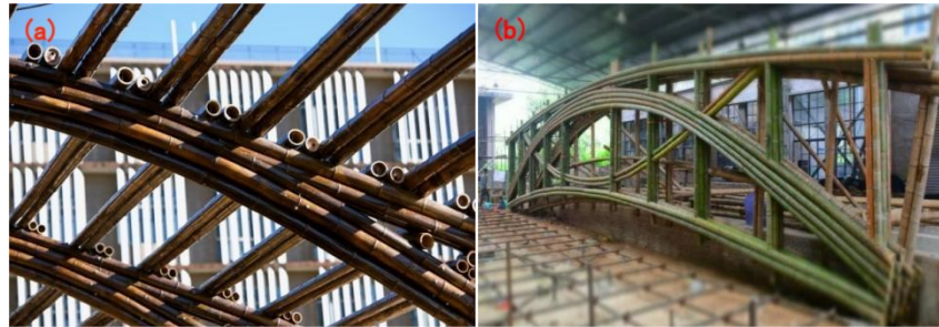
Fig. 4. (a) Round bamboo arch, (b) round bamboo trusses
