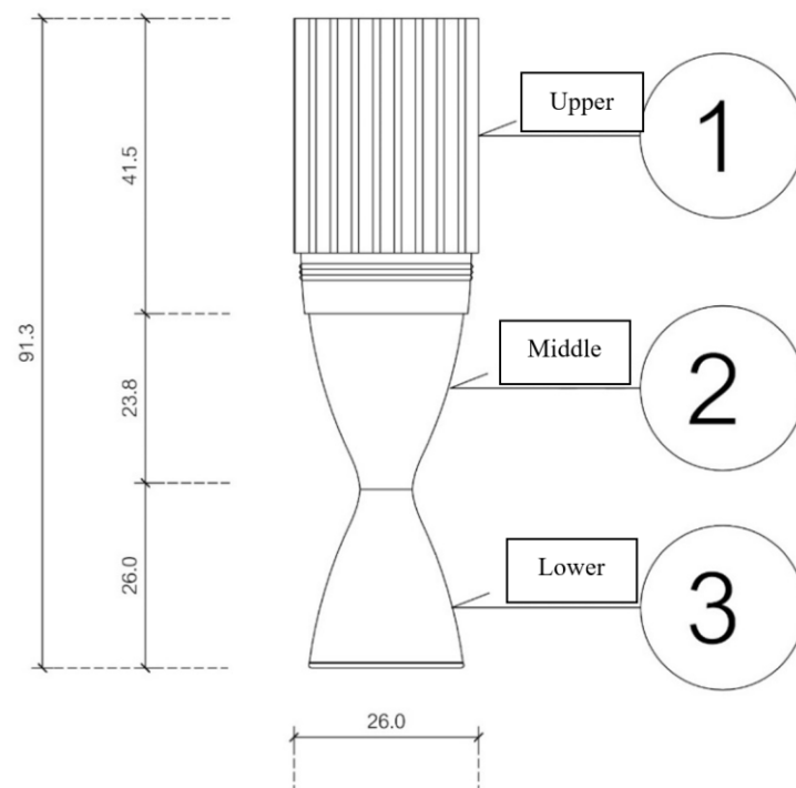
Fig. 4. The drum components are divided into three parts and the unit used for each measurement is “cm”
