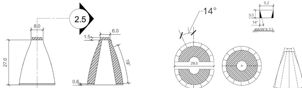
Fig. 7a. Lower part of the drum Note: All measurements are in unit “cm”.
