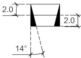
Fig. 5a. Upper part of drum Fig. 5b. Wood angle of 14^\circ Note: All measurements are in unit “cm”.
