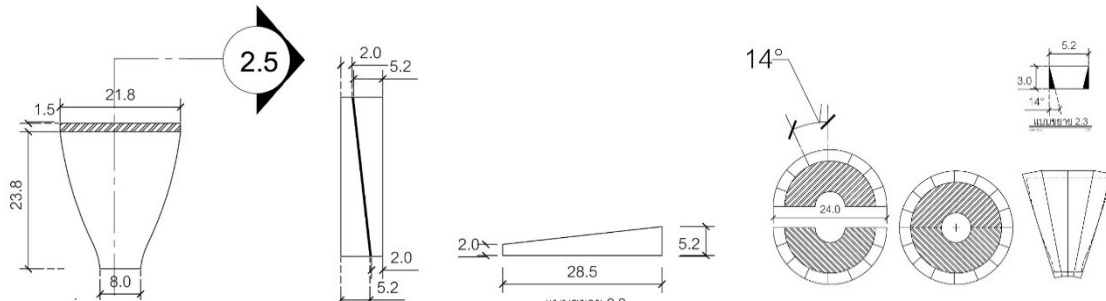
Fig. 6a. Middle of the drum Fig. 6b. Saw the two pieces Note: All measurements are in unit “cm”.
