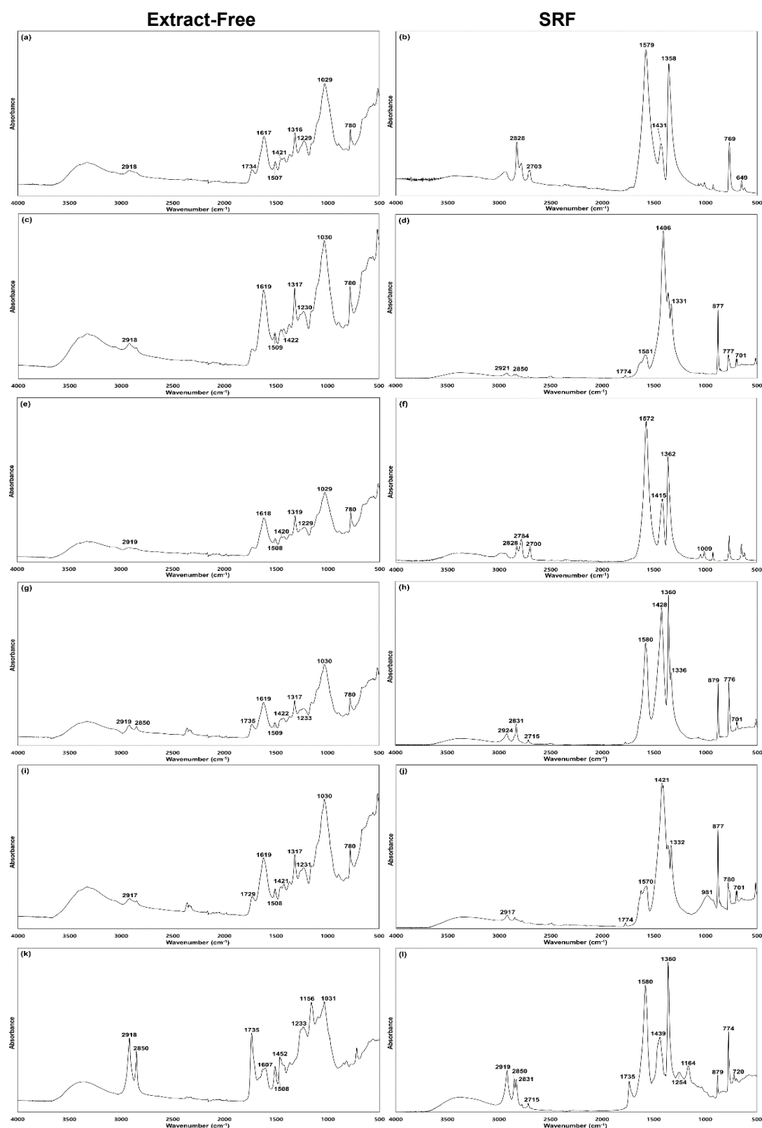
Fig. 3. FT-IR spectra of EF and SRF isolated from six Korean Quercus species: a) and b) Q. acutissima ; c) and d) Q. aliena , e) and f) Q. dentata , g) and h) Q. mongolica , i) and j) Q. serrata , and k) and l) Q. variabilis
