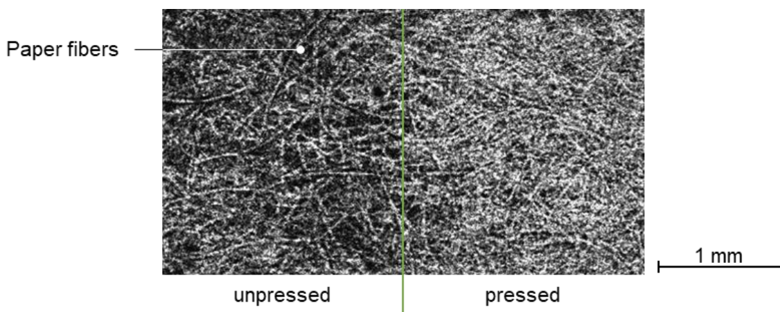
Fig. 10. Computed tomography images of samples before and after pressing (Stein 2019)
