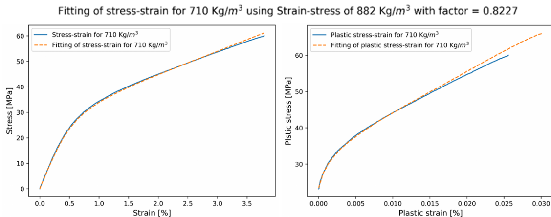
Fig. 11. Efficiency factor of the (plastic) stress-strain curve of 710 \text{ kg/m}^3 using of 882 \text{ kg/m}^3 as a reference
