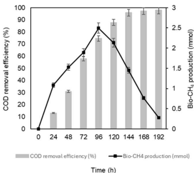
Fig. 4. Production of Bio- \text{CH}_4 and COD removal, in batch reactors, at an initial substrate concentration (20.1 g/L \text{O}_2 ) with a fermentation time of 192 h
