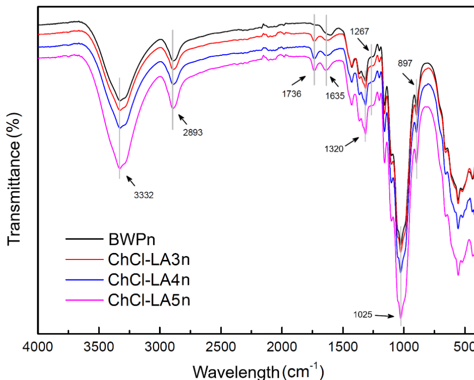
Fig. 1. FT-IR spectra of BWPn, ChCl-LA3n, ChCl-LA4n and ChCl-LA5n samples
