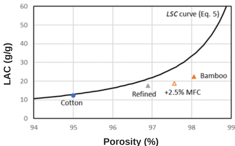
Fig. 5. Liquid absorbency capacity ( LAC ) as a function of porosity for all types of foam and evolution of theoretical liquid storage capacity ( LSC ) of the porous structure according to Eq. 5
