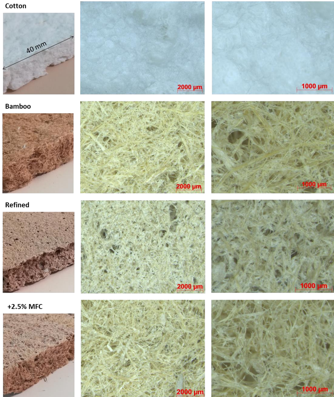
Fig. 4. Pictures of solid foams and surface structures imaged by optical microscopy
