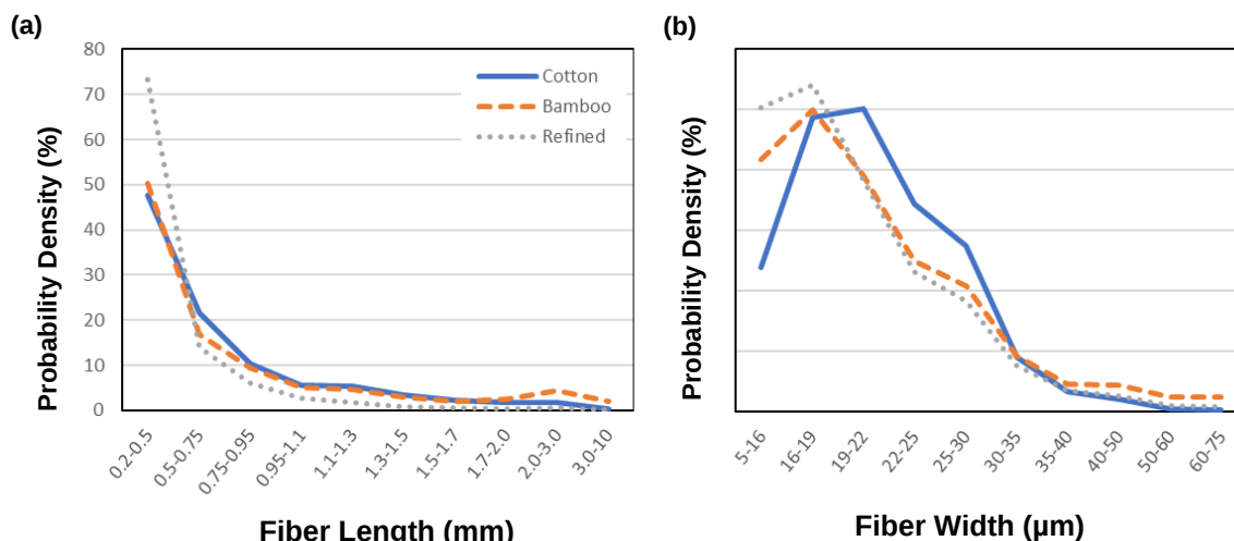
Fig. 3. Distributions in (a) length and (b) width of cotton, bamboo and refined bamboo fibers
